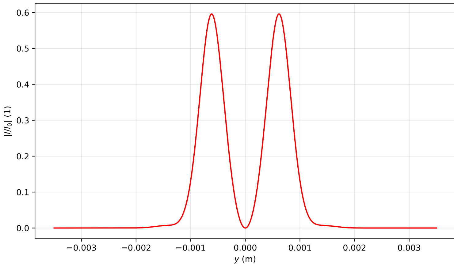
Intensity profile I(x=0, y, z=1.194)/I_0 , P_{in}=3.0P_{cr} , artificial time
